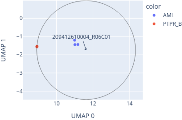
Close-up of UMAP for 209412610004_R06C01 reference: AllIDATv2_20210804_HPAP_Sarc.xlsx (19967 cases), 0 CpGs
