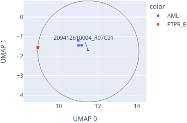
Close-up of UMAP for 209412610004_R07C01 reference: AllIDATv2_20210804_HPAP_Sarc.xlsx (19967 cases), 0 CpGs
