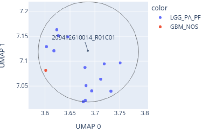
Close-up of UMAP for 209412610014_R01C01 reference: AllIDATv2_20210804_HPAP_Sarc.xlsx (19967 cases), 0 CpGs
