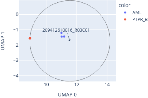
Close-up of UMAP for 209412610016_R03C01 reference: AllIDATv2_20210804_HPAP_Sarc.xlsx (19967 cases), 0 CpGs
