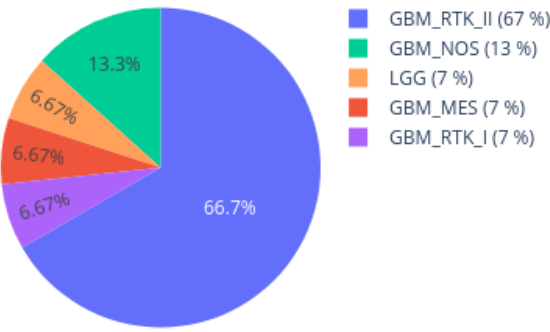
Neighbors in UMAP for 209412610018_R01C01 reference: AllIDATv2_20210804_HPAP_Sarc.xlsx (19967 cases), 0 CpGs
