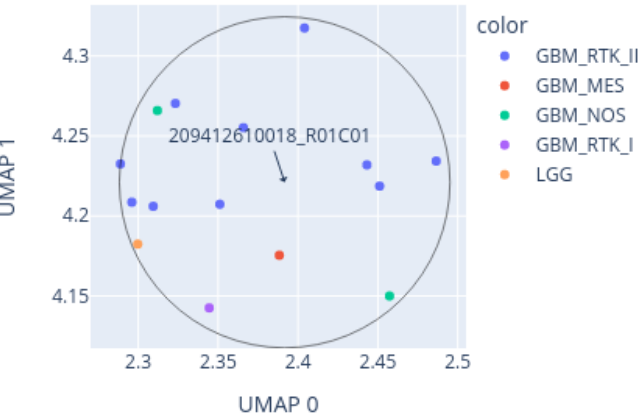
Close-up of UMAP for 209412610018_R01C01 reference: AllIDATv2_20210804_HPAP_Sarc.xlsx (19967 cases), 0 CpGs
