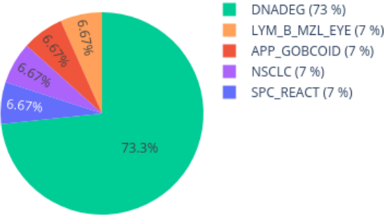
Neighbors in UMAP for 209412610019_R03C01 reference: AllIDATv2_20210804_HPAP_Sarc.xlsx (19967 cases), 0 CpGs
