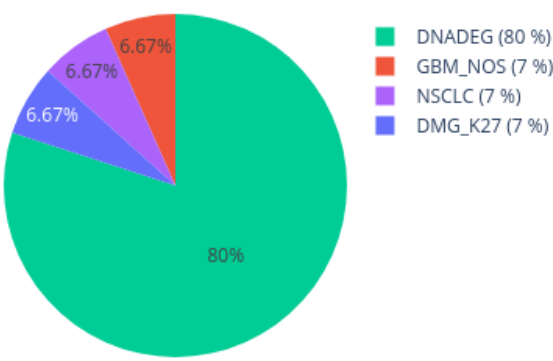
Neighbors in UMAP for 209412610020_R07C01 reference: AllIDATv2_20210804_HPAP_Sarc.xlsx (19967 cases), 0 CpGs
