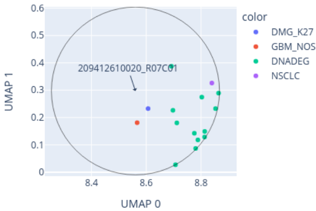
Close-up of UMAP for 209412610020_R07C01 reference: AllIDATv2_20210804_HPAP_Sarc.xlsx (19967 cases), 0 CpGs
