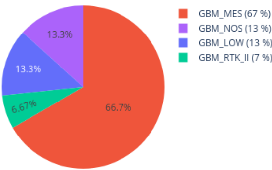
Neighbors in UMAP for 209412610023_R05C01 reference: AllIDATv2_20210804_HPAP_Sarc.xlsx (19967 cases), 0 CpGs
