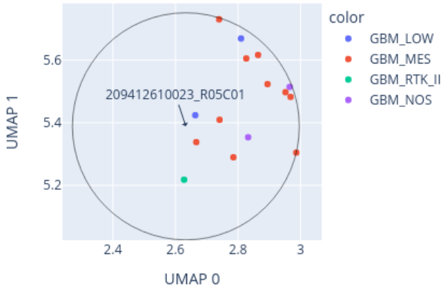
Close-up of UMAP for 209412610023_R05C01 reference: AllIDATv2_20210804_HPAP_Sarc.xlsx (19967 cases), 0 CpGs
