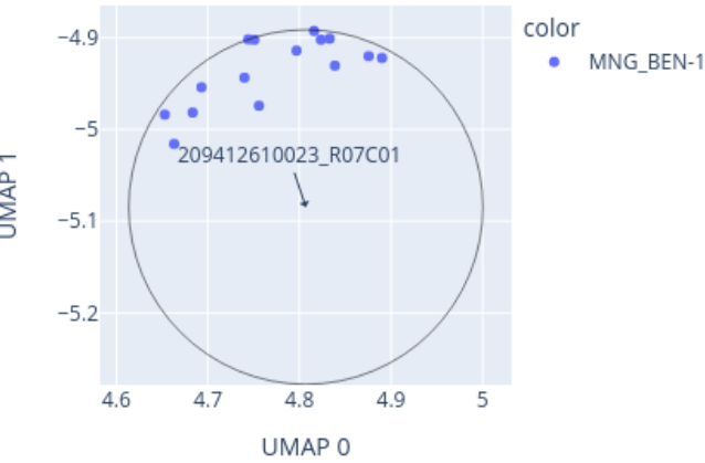
Close-up of UMAP for 209412610023_R07C01 reference: AllIDATv2_20210804_HPAP_Sarc.xlsx (19967 cases), 0 CpGs
