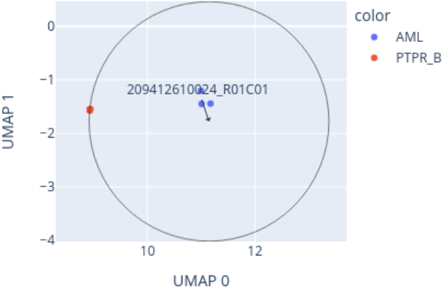
Close-up of UMAP for 209412610024_R01C01 reference: AllIDATv2_20210804_HPAP_Sarc.xlsx (19967 cases), 0 CpGs
