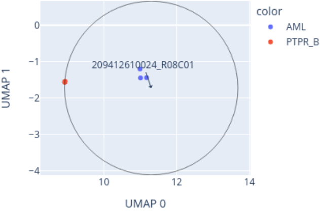
Close-up of UMAP for 209412610024_R08C01 reference: AllIDATv2_20210804_HPAP_Sarc.xlsx (19967 cases), 0 CpGs
