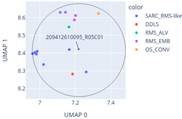
Close-up of UMAP for 209412610095_R05C01 reference: AllIDATv2_20210804_HPAP_Sarc.xlsx (19967 cases), 0 CpGs
