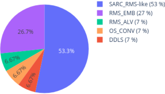
Neighbors in UMAP for 209412610095_R05C01 reference: AllIDATv2_20210804_HPAP_Sarc.xlsx (19967 cases), 0 CpGs
