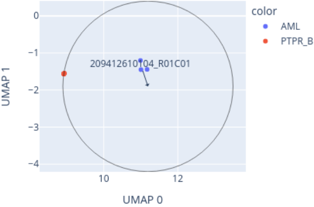
Close-up of UMAP for 209412610104_R01C01 reference: AllIDATv2_20210804_HPAP_Sarc.xlsx (19967 cases), 0 CpGs
