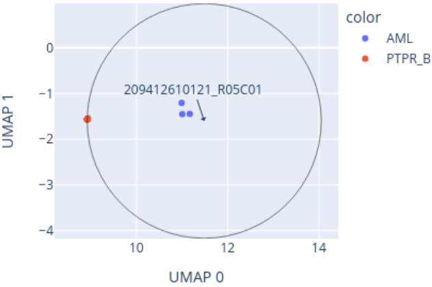
Close-up of UMAP for 209412610121_R05C01 reference: AllIDATv2_20210804_HPAP_Sarc.xlsx (19967 cases), 0 CpGs
