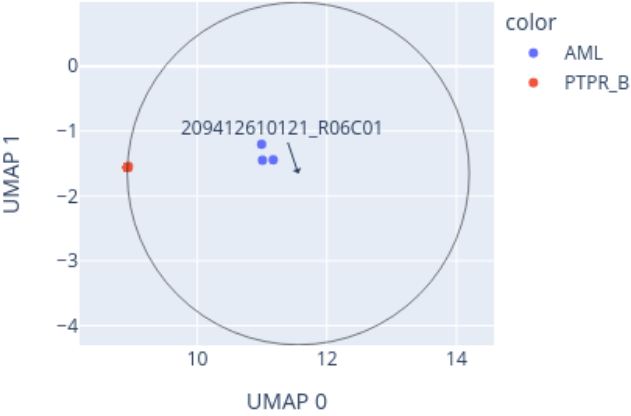
Close-up of UMAP for 209412610121_R06C01 reference: AllIDATv2_20210804_HPAP_Sarc.xlsx (19967 cases), 0 CpGs
