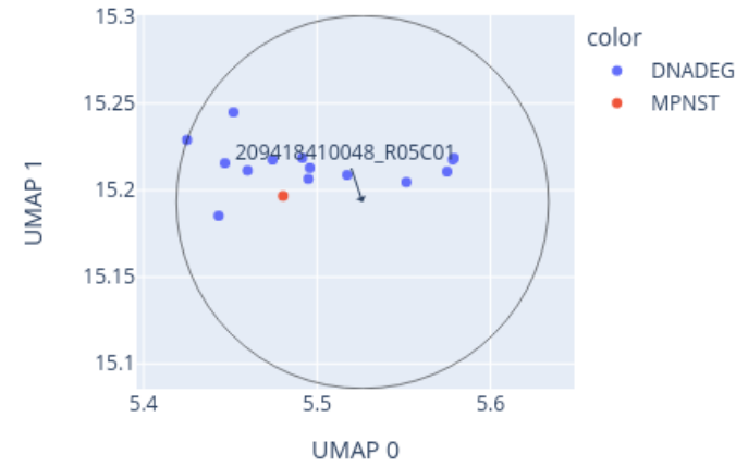
Close-up of UMAP for 209418410048_R05C01 reference: AllIDATv2_20210804_HPAP_Sarc.xlsx (19967 cases), 0 CpGs
