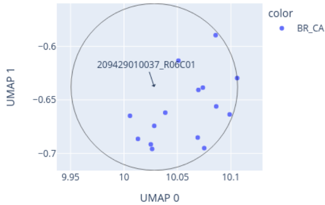
Close-up of UMAP for 209429010037_R06C01 reference: AllIDATv2_20210804_HPAP_Sarc.xlsx (19967 cases), 0 CpGs
