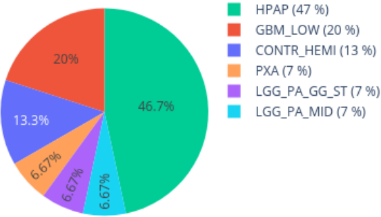
Neighbors in UMAP for 209429010053_R04C01 reference: AllIDATv2_20210804_HPAP_Sarc.xlsx (19967 cases), 0 CpGs
