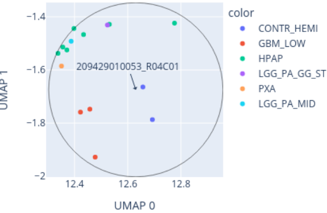
Close-up of UMAP for 209429010053_R04C01 reference: AllIDATv2_20210804_HPAP_Sarc.xlsx (19967 cases), 0 CpGs
