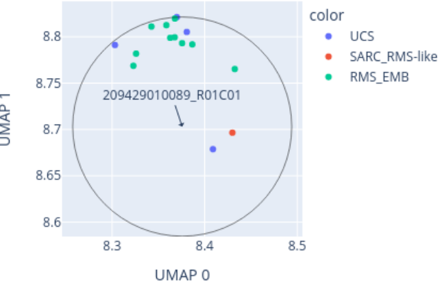
Close-up of UMAP for 209429010089_R01C01 reference: AllIDATv2_20210804_HPAP_Sarc.xlsx (19967 cases), 0 CpGs
