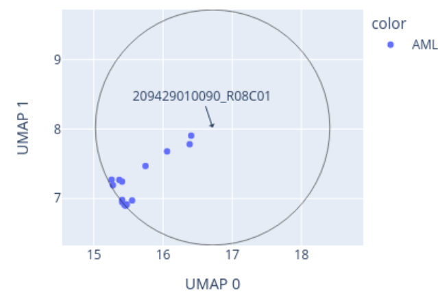
Close-up of UMAP for 209429010090_R08C01 reference: AllIDATv2_20210804_HPAP_Sarc.xlsx (19967 cases), 0 CpGs
