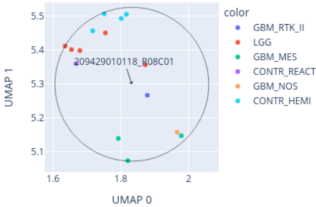
Close-up of UMAP for 209429010118_R08C01 reference: AllIDATv2_20210804_HPAP_Sarc.xlsx (19967 cases), 0 CpGs
