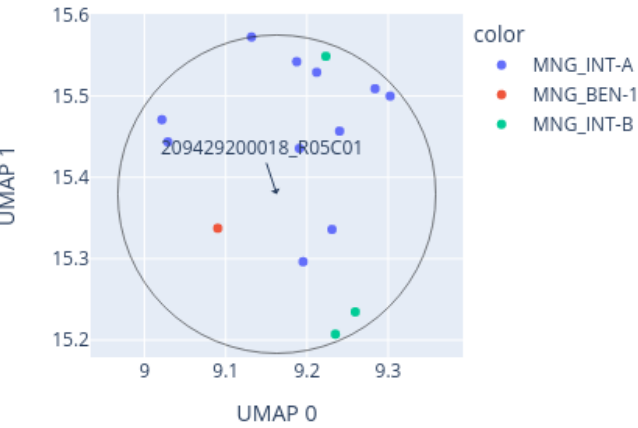
Close-up of UMAP for 209429200018_R05C01 reference: AllIDATv2_20210804_HPAP_Sarc.xlsx (19967 cases), 0 CpGs
