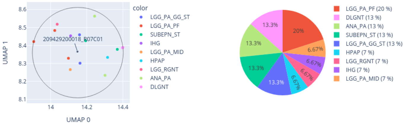
Close-up of UMAP for 209429200018_R07C01 reference: AllIDATv2_20210804_HPAP_Sarc.xlsx (19967 cases), 0 CpGs
