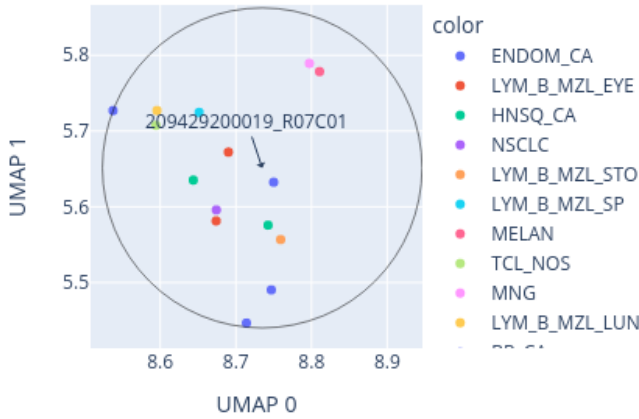
Close-up of UMAP for 209429200019_R07C01 reference: AllIDATv2_20210804_HPAP_Sarc.xlsx (19967 cases), 0 CpGs
