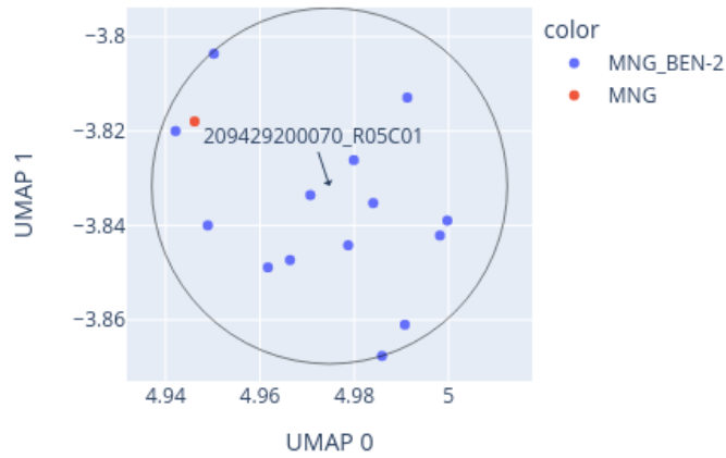
Close-up of UMAP for 209429200070_R05C01 reference: AllIDATv2_20210804_HPAP_Sarc.xlsx (19967 cases), 0 CpGs
