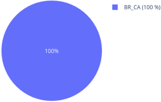
Neighbors in UMAP for 209429200070_R06C01 reference: AllIDATv2_20210804_HPAP_Sarc.xlsx (19967 cases), 0 CpGs
