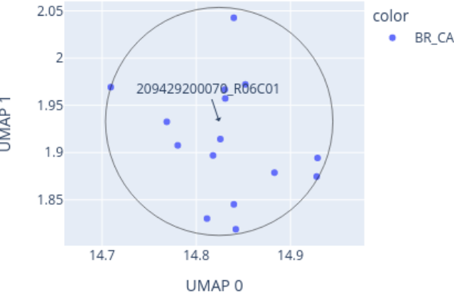
Close-up of UMAP for 209429200070_R06C01 reference: AllIDATv2_20210804_HPAP_Sarc.xlsx (19967 cases), 0 CpGs
