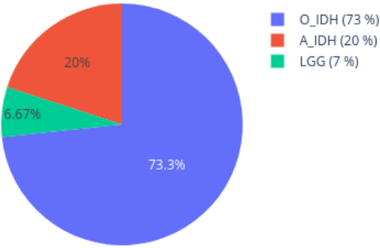
Neighbors in UMAP for 209429200152_R02C01 reference: AllIDATv2_20210804_HPAP_Sarc.xlsx (19967 cases), 0 CpGs
