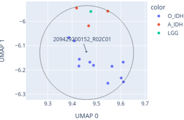
Close-up of UMAP for 209429200152_R02C01 reference: AllIDATv2_20210804_HPAP_Sarc.xlsx (19967 cases), 0 CpGs
