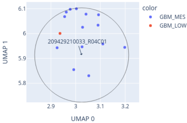
Close-up of UMAP for 209429210033_R04C01 reference: AllIDATv2_20210804_HPAP_Sarc.xlsx (19967 cases), 0 CpGs
