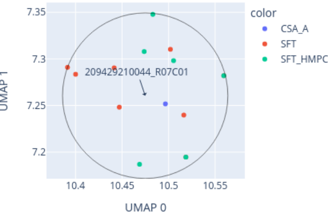
Close-up of UMAP for 209429210044_R07C01 reference: AllIDATv2_20210804_HPAP_Sarc.xlsx (19967 cases), 0 CpGs
