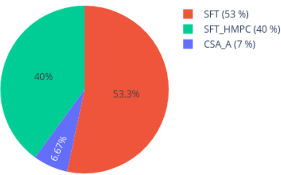
Neighbors in UMAP for 209429210044_R07C01 reference: AllIDATv2_20210804_HPAP_Sarc.xlsx (19967 cases), 0 CpGs
