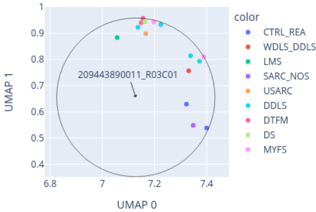
Close-up of UMAP for 209443890011_R03C01 reference: AllIDATv2_20210804_HPAP_Sarc.xlsx (19967 cases), 0 CpGs
