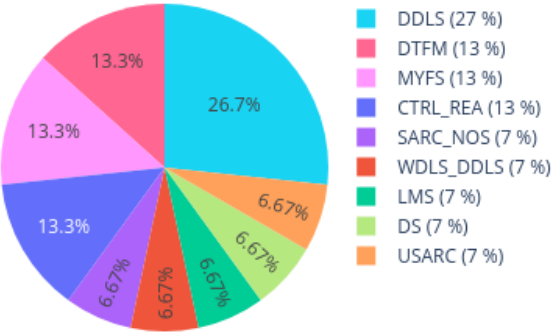
Neighbors in UMAP for 209443890011_R03C01 reference: AllIDATv2_20210804_HPAP_Sarc.xlsx (19967 cases), 0 CpGs
