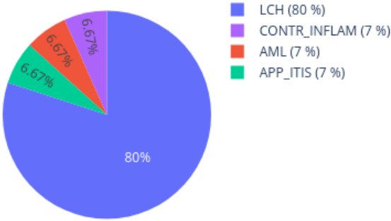
Neighbors in UMAP for 209443890012_R01C01 reference: AllIDATv2_20210804_HPAP_Sarc.xlsx (19967 cases), 0 CpGs
