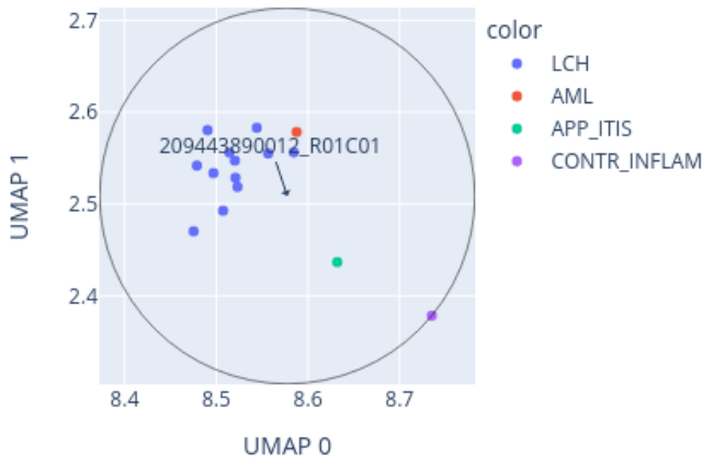
Close-up of UMAP for 209443890012_R01C01 reference: AllIDATv2_20210804_HPAP_Sarc.xlsx (19967 cases), 0 CpGs
