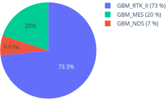
Neighbors in UMAP for 209443890012_R02C01 reference: AllIDATv2_20210804_HPAP_Sarc.xlsx (19967 cases), 0 CpGs
