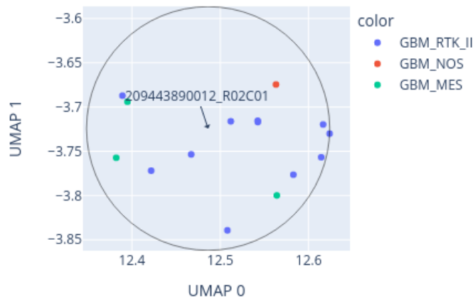
Close-up of UMAP for 209443890012_R02C01 reference: AllIDATv2_20210804_HPAP_Sarc.xlsx (19967 cases), 0 CpGs
