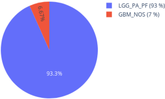
Neighbors in UMAP for 209443890017_R01C01 reference: AllIDATv2_20210804_HPAP_Sarc.xlsx (19967 cases), 0 CpGs
