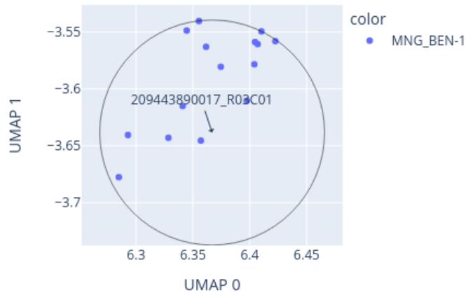
Close-up of UMAP for 209443890017_R03C01 reference: AllIDATv2_20210804_HPAP_Sarc.xlsx (19967 cases), 0 CpGs
