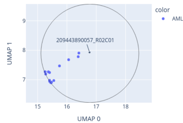
Close-up of UMAP for 209443890057_R02C01 reference: AllIDATv2_20210804_HPAP_Sarc.xlsx (19967 cases), 0 CpGs
