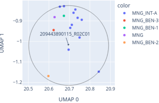
Close-up of UMAP for 209443890115_R02C01 reference: AllIDATv2_20210804_HPAP_Sarc.xlsx (19967 cases), 0 CpGs
