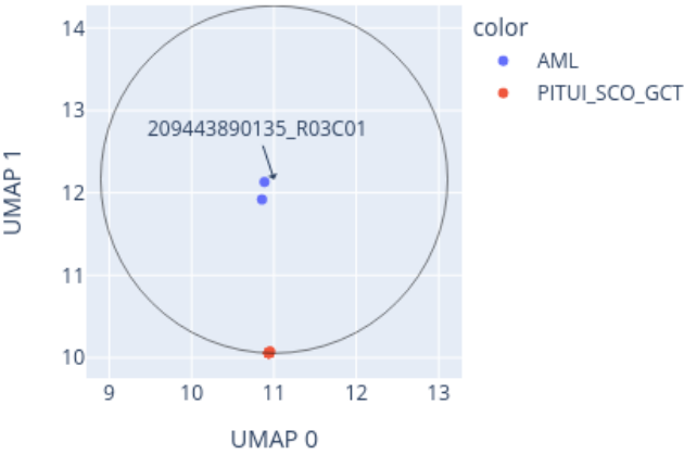
Close-up of UMAP for 209443890135_R03C01 reference: AllIDATv2_20210804_HPAP_Sarc.xlsx (19967 cases), 0 CpGs
