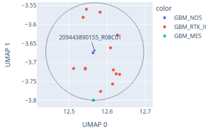
Close-up of UMAP for 209443890155_R08C01 reference: AllIDATv2_20210804_HPAP_Sarc.xlsx (19967 cases), 0 CpGs
