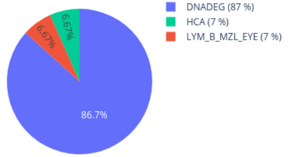
Neighbors in UMAP for 210238430011_R03C01 reference: AllIDATv2_20210804_HPAP_Sarc.xlsx (19967 cases), 0 CpGs
