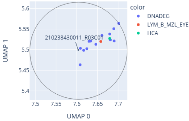
Close-up of UMAP for 210238430011_R03C01 reference: AllIDATv2_20210804_HPAP_Sarc.xlsx (19967 cases), 0 CpGs
