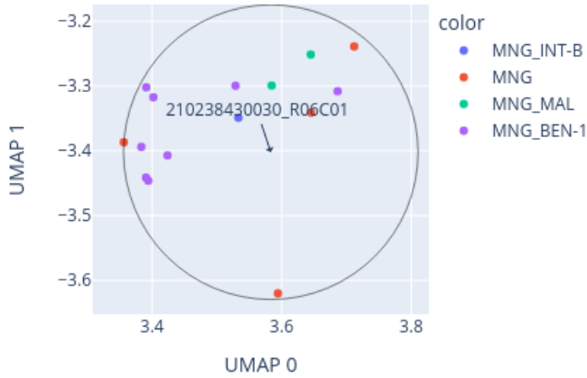
Close-up of UMAP for 210238430030_R06C01 reference: AllIDATv2_20210804_HPAP_Sarc.xlsx (19967 cases), 0 CpGs
