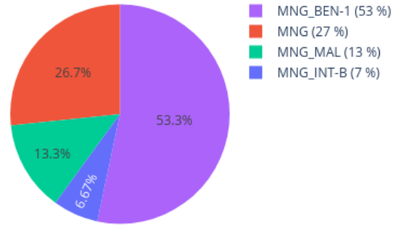
Neighbors in UMAP for 210238430030_R06C01 reference: AllIDATv2_20210804_HPAP_Sarc.xlsx (19967 cases), 0 CpGs
