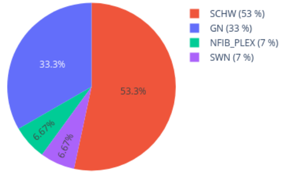
Neighbors in UMAP for 210238430061_R02C01 reference: AllIDATv2_20210804_HPAP_Sarc.xlsx (19967 cases), 0 CpGs
