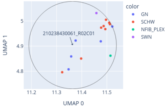
Close-up of UMAP for 210238430061_R02C01 reference: AllIDATv2_20210804_HPAP_Sarc.xlsx (19967 cases), 0 CpGs
