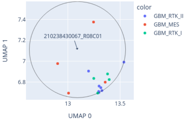
Close-up of UMAP for 210238430067_R08C01 reference: GSE90496_lfp02.xlsx (2980 cases), 0 CpGs
