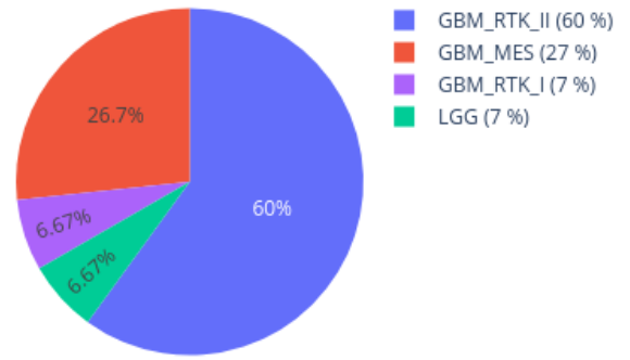
Neighbors in UMAP for 210238430083_R05C01 reference: AllIDATv2_20210804_HPAP_Sarc.xlsx (19967 cases), 0 CpGs
