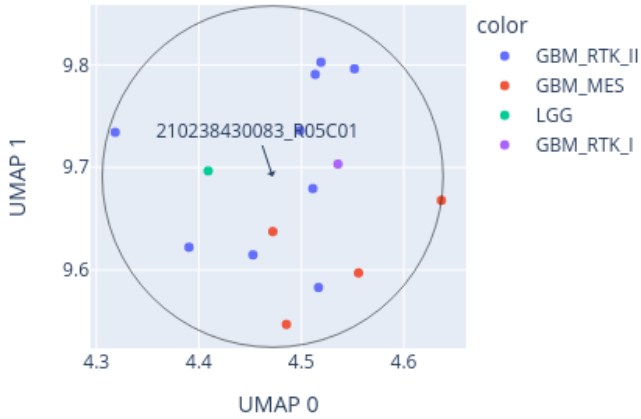
Close-up of UMAP for 210238430083_R05C01 reference: AllIDATv2_20210804_HPAP_Sarc.xlsx (19967 cases), 0 CpGs
