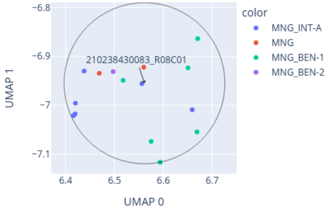
Close-up of UMAP for 210238430083_R08C01 reference: AllIDATv2_20210804_HPAP_Sarc.xlsx (19967 cases), 0 CpGs
