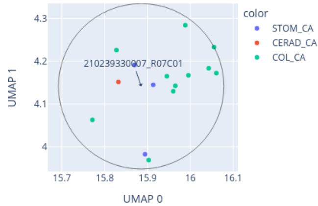
Close-up of UMAP for 210239330007_R07C01 reference: AllIDATv2_20210804_HPAP_Sarc.xlsx (19967 cases), 0 CpGs
