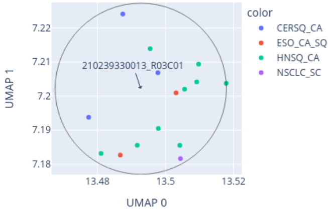
Close-up of UMAP for 210239330013_R03C01 reference: AllIDATv2_20210804_HPAP_Sarc.xlsx (19967 cases), 0 CpGs
