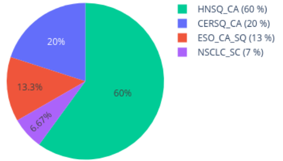
Neighbors in UMAP for 210239330013_R03C01 reference: AllIDATv2_20210804_HPAP_Sarc.xlsx (19967 cases), 0 CpGs
