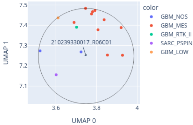
Close-up of UMAP for 210239330017_R06C01 reference: AllIDATv2_20210804_HPAP_Sarc.xlsx (19967 cases), 0 CpGs
