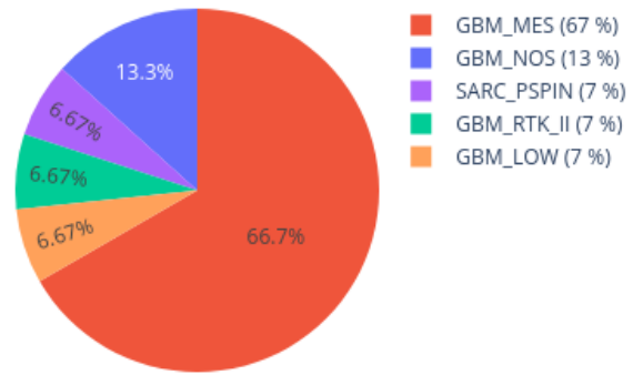
Neighbors in UMAP for 210239330017_R06C01 reference: AllIDATv2_20210804_HPAP_Sarc.xlsx (19967 cases), 0 CpGs
