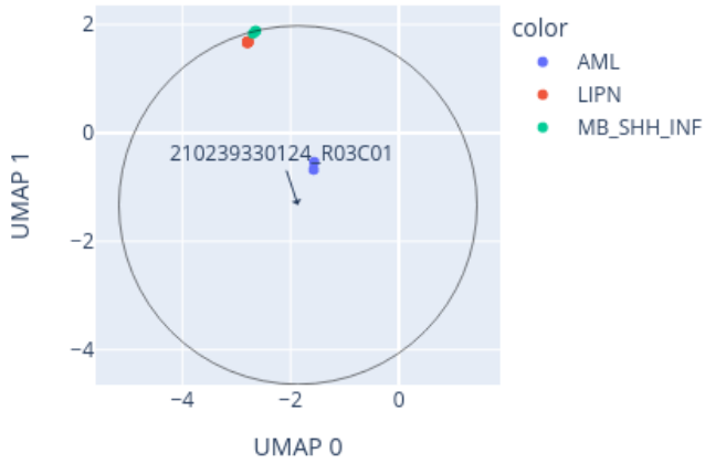
Close-up of UMAP for 210239330124_R03C01 reference: AllIDATv2_20210804_HPAP_Sarc.xlsx (19967 cases), 0 CpGs
