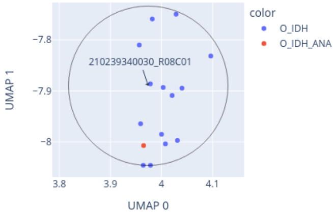
Close-up of UMAP for 210239340030_R08C01 reference: AllIDATv2_20210804_HPAP_Sarc.xlsx (19967 cases), 0 CpGs
