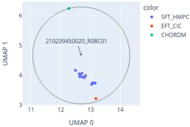
Close-up of UMAP for 210239450020_R08C01 reference: GSE90496_lfP02.xlsx (2980 cases), 0 CpGs
