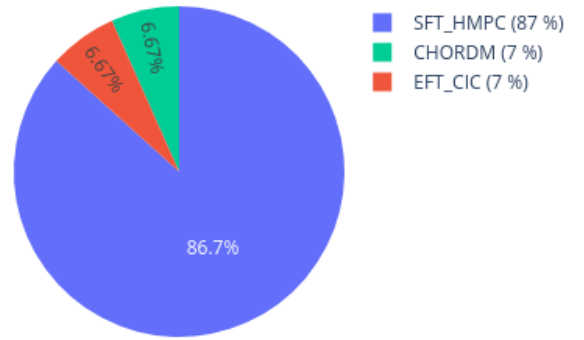
Neighbors in UMAP for 210239450020_R08C01 reference: GSE90496_lfP02.xlsx (2980 cases), 0 CpGs
